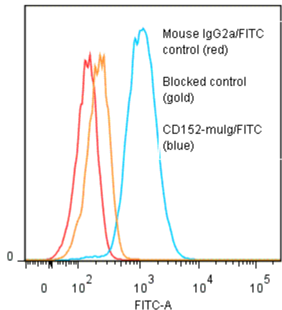
Binding of CD152-mulg/FITC to human Raji cells
