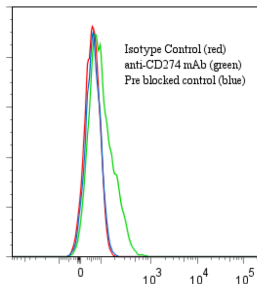
Binding of anti-CD274(B7-H1) mAb + GAM/FITC to stimulated human PBMC
