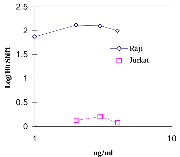
Binding of anti-CD75 antibody to human cell lines
