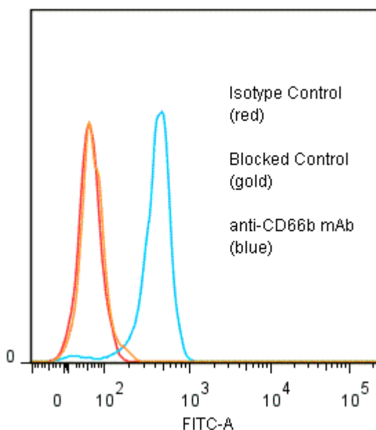
Binding of anti-CD66(ANC4A4) antibody +GAM/FITC to human PMN
