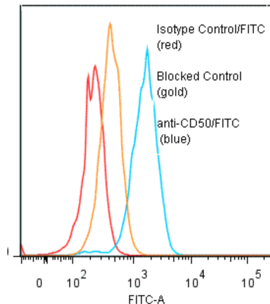
Binding of anti-CD50/FITC to human Jurkat cells
