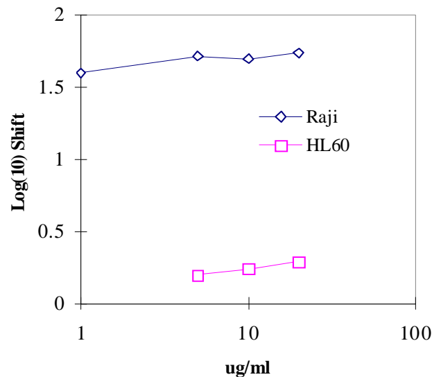
Binding of anti-CD38 antibody to human cell lines
