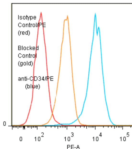
Binding of anti-CD34/PE to human KG1 cells
