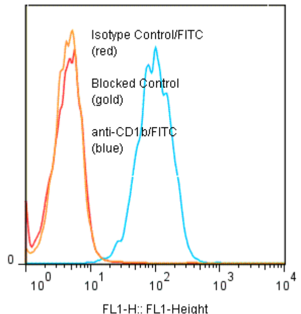
Binding of anti-CD1b/FITC to human HPB-MLT cells
